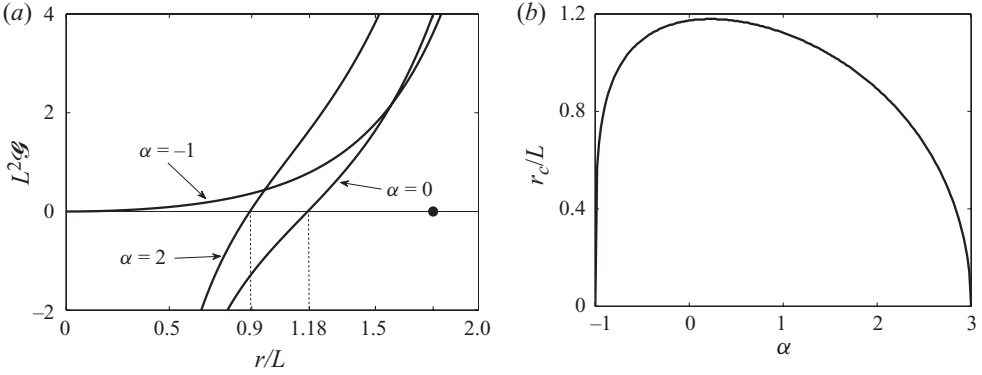
FIGURE 3. (a) The function \mathcal{G}(r; \alpha) given in (1.4) and non-dimensionalized with L^2 , for the Lamb–Oseen vortex and \alpha = -1 , 0 and \alpha = 2 . For \alpha = -1 and \alpha = 3 (not shown) \mathcal{G} \geq 0 for all r . For \alpha = 0 we have \mathcal{G} > 0 for all r/L > r_c/L \approx 1.18 . (b) Graph showing the critical radius r_c/L as a function of \alpha \in [-1, 3] . The greatest value is found for \alpha \approx 0.2 with r_c/L \approx 1.19 . There are no \alpha values for which \mathcal{G} \leq 0 for all r so (1.4) is never satisfied on the unbounded domain. The symbol \bullet is at the position r/L = r_c/L \approx 1.79 from figure 3.
